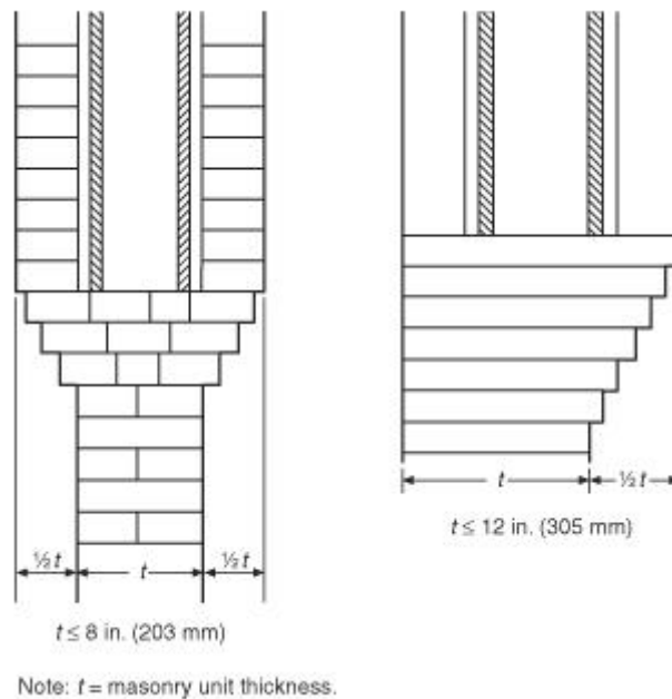
FIGURE 7.1.2(a) Corbels for Supporting Chimneys.
