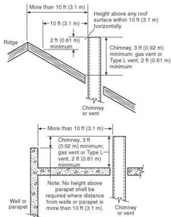
FIGURE 4.2(b) Chimney or Vent Termination More Than 10 ft (3.1 m) from Ridge, Wall, or Parapet. Copyright NFPA
