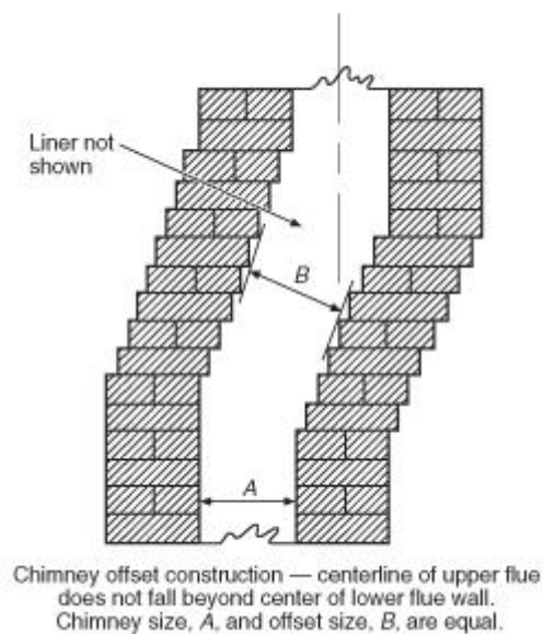
FIGURE 7.1.2(b) Corbels to Change Chimney Direction.
