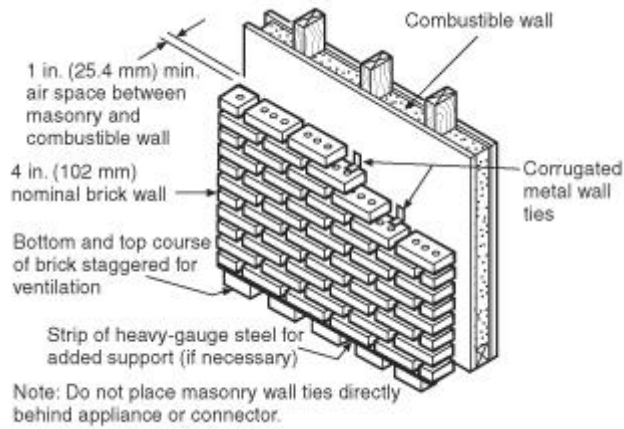
FIGURE 12.6.2.1(c) Masonry Clearance Reduction System.
