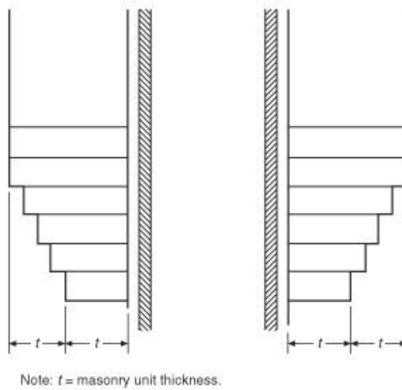
FIGURE 7.1.2(c) Corbels to Increase Chimney Wall Thickness.
