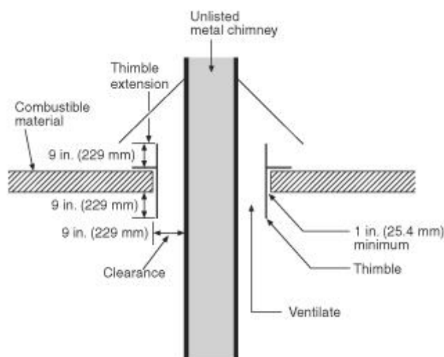
FIGURE 8.2.2.2.7 Ventilating Thimble.
